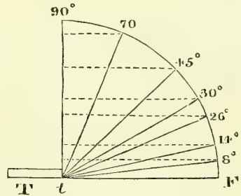
Insertion of Fibres into Tendon.
